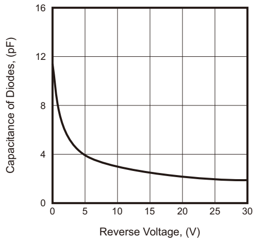
Fig.3 - Capacitance of Diodes
